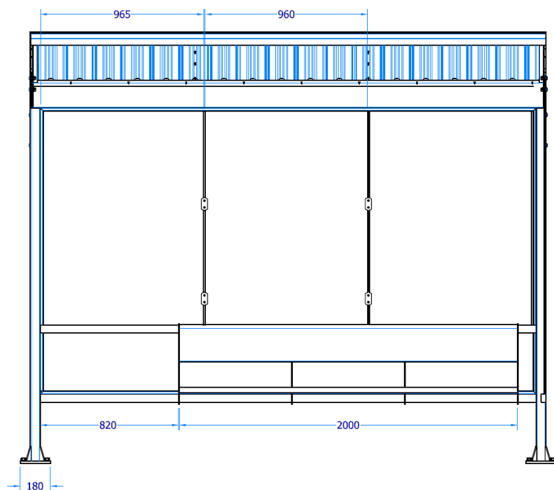
ABRIGO 2,0 X 3,00m - VISTA FRONTAL
